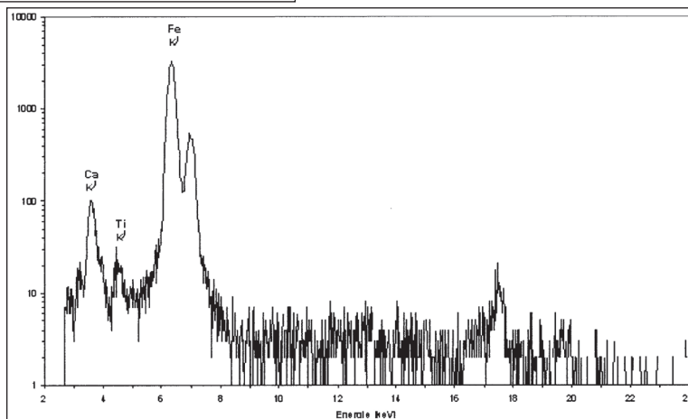
Obr. 11: XRF spektrum povrhu strusky 102/6
