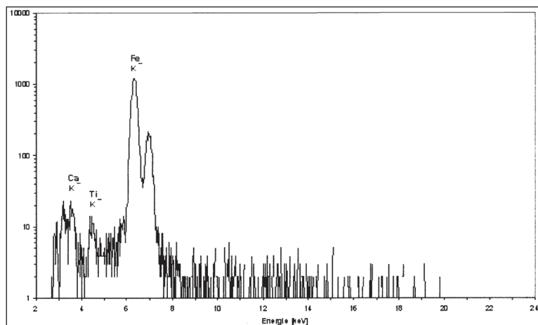
Obr. 11: XRF spektrum povrhu strusky 102/6
